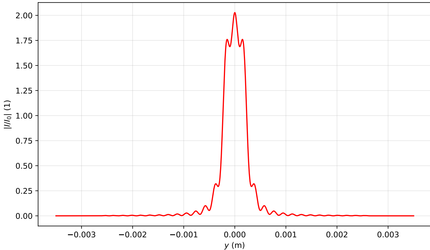
Intensity profile I(x=0, y, z=0.159)/I_0 , P_{in}=2.0P_{cr} , artificial time
